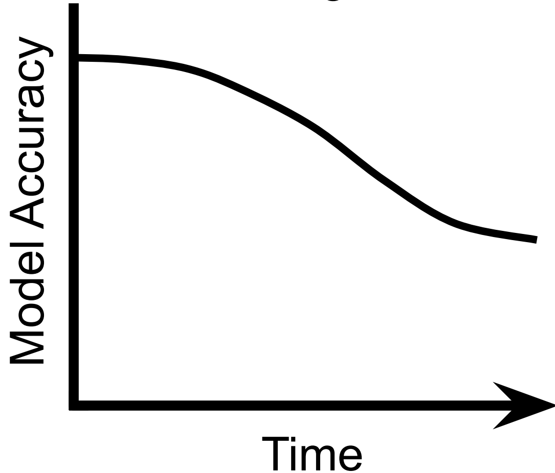
Model Degradation
