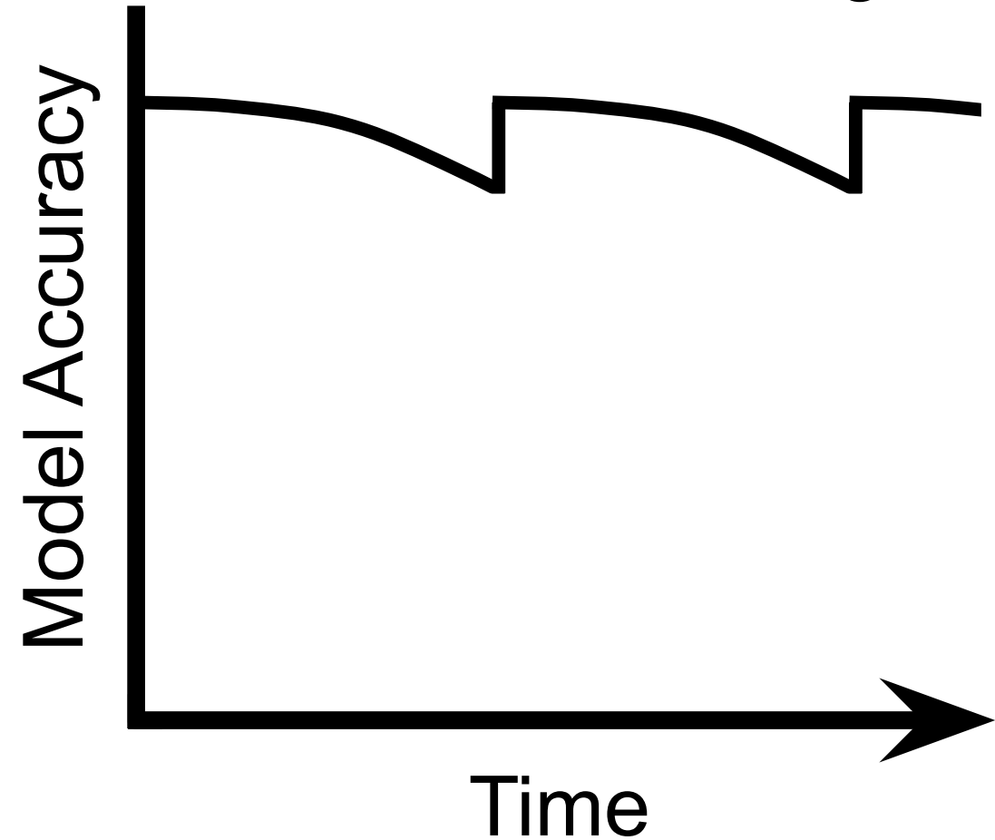
Model Retraining
